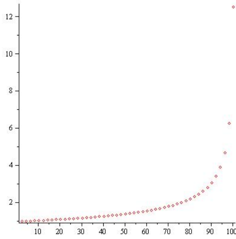
FIGURE 1. \mathbb{E}_e^{(100)} Y_k for k = 2, 4, \dots, 100
