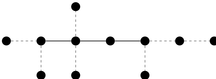
Figure 4.5: A tree decomposed into its trunk (with thick edges) and twigs (represented by dashed edges).
