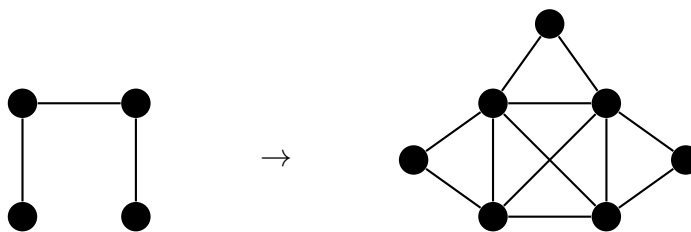
Figure 4.1: An example of the split graph construction
