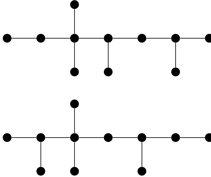
Figure 4.4: 11-vertex trees with the same generalized degree sequence
