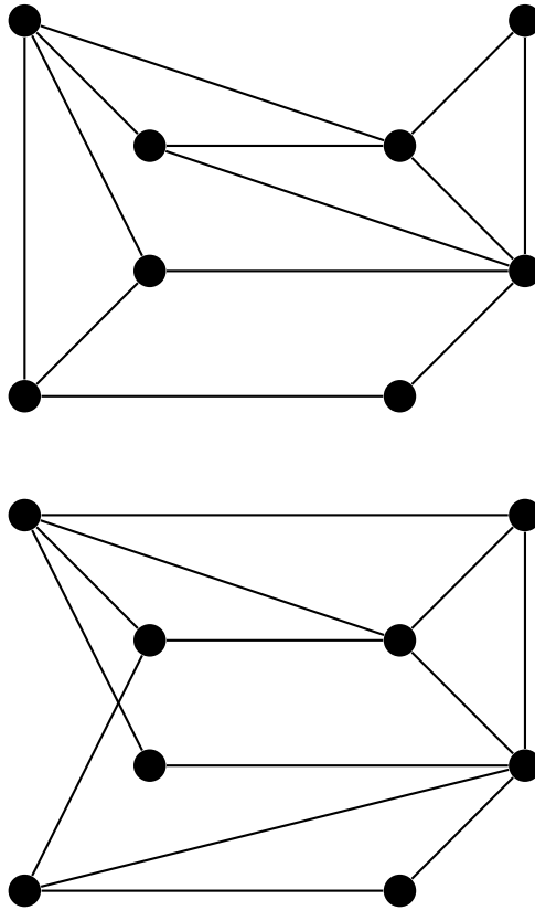
Figure 4.3: 8-vertex graphs with the same generalized degree sequence
