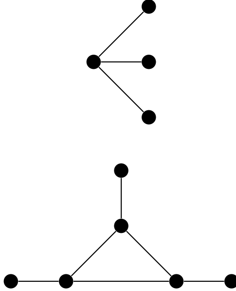
Figure 3.1: The claw (top) and the net (bottom), small graphs that are not e -positive.
