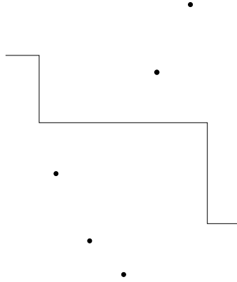
FIGURE 4. A section D of width 5 and a D -standard placement of rooks (rooks outside of D are not pictured).
