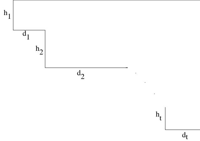
FIGURE 11. The Ferrers board B(h_1, d_1; \dots; h_t, d_t) , where d_i \in \mathbb{P}, h_i \in \mathbb{N} for 1 \leq i \leq t . The first d_1 columns have height h_1 , the next d_2 have height h_1 + h_2 , etc.
