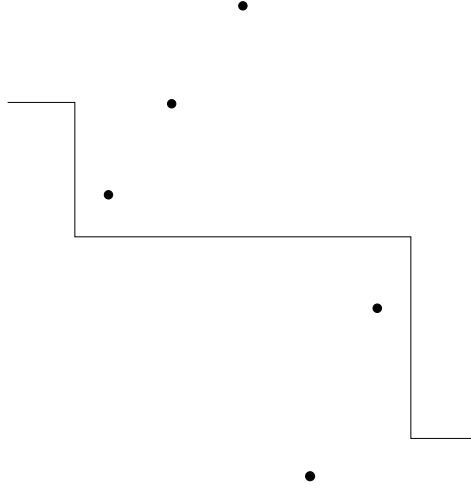
FIGURE 12. A section D of width 5 and a D -regular placement of rooks (rooks outside of D are not pictured).
