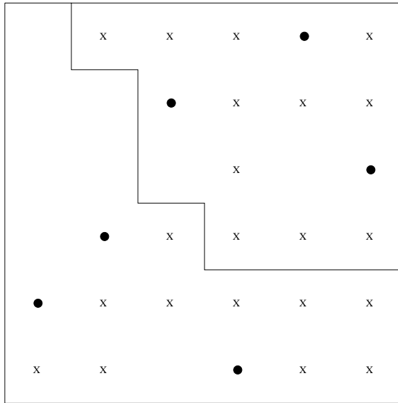
FIGURE 3. A placement of 6 rooks with 3 rooks on B : \text{cross} = 27 so \text{mat} = 3 * 6 + 16 - 27 = 7 .
