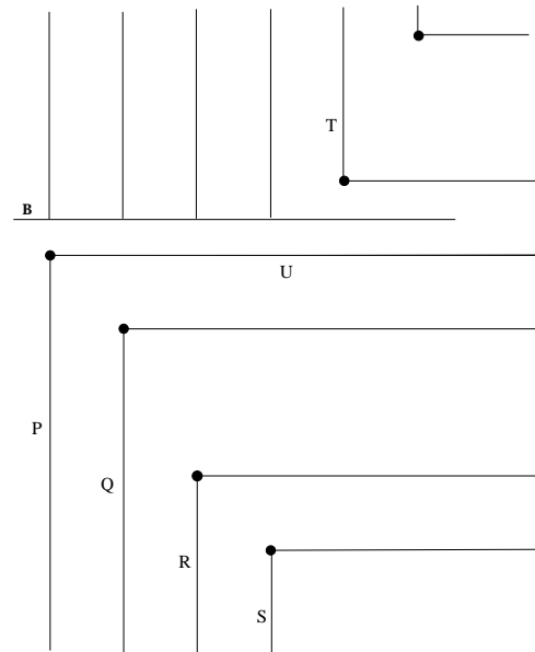
FIGURE 6. Another D semi-standard placement of rooks. The left-rook has moved down to row j_{p+1} .
