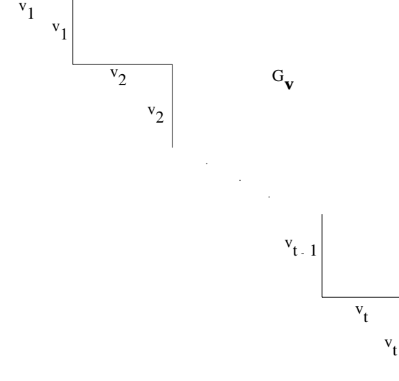
FIGURE 14. The Ferrers board G_{\mathbf{v}} . The first v_1 columns are empty, the next v_2 have height v_1 , etc.
