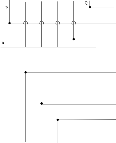
FIGURE 8. Another D semi-standard placement of rooks. The left-rook has moved up to row i_1 .
