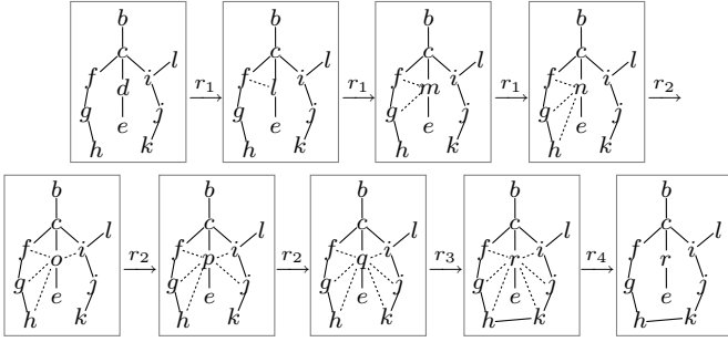
Fig. 12. A partial trajectory arising from the MakeGraph rules for a particular graph.
