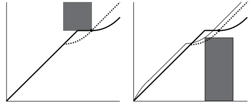
Fig. 6. The dotted line on the right indicates a collision path; the thin line is modified to avoid the collision by modifying the robot on the z -axis.
