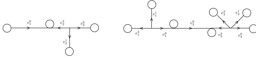
Figure 8. G_{(1,2)} [left]; G_{(2,1,3)} [right].
