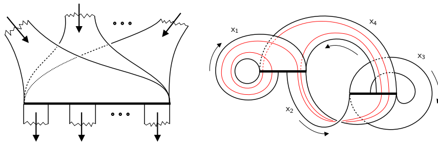
Figure 2. A branchline chart for a template [left]; an example of a template with an unknotted periodic orbit on it [right]. In the alphabet \{x_1, x_2, x_3, x_4\} , this knot corresponds to the word (x_1^2(x_2x_4)^2) = (x_1x_1x_2x_4x_2x_4) .
